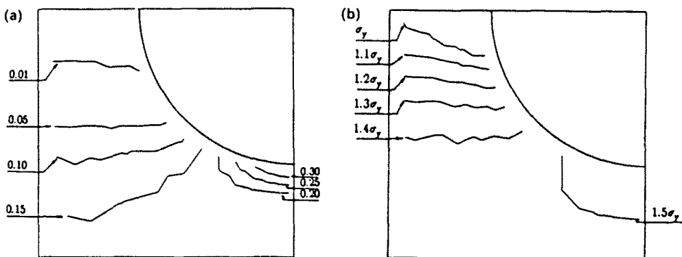
Fig. 6. Contours of constant von Mises stresses and corresponding strain contours for a shear deformed material at \gamma = 0.20 ( f = 0.28 ).
